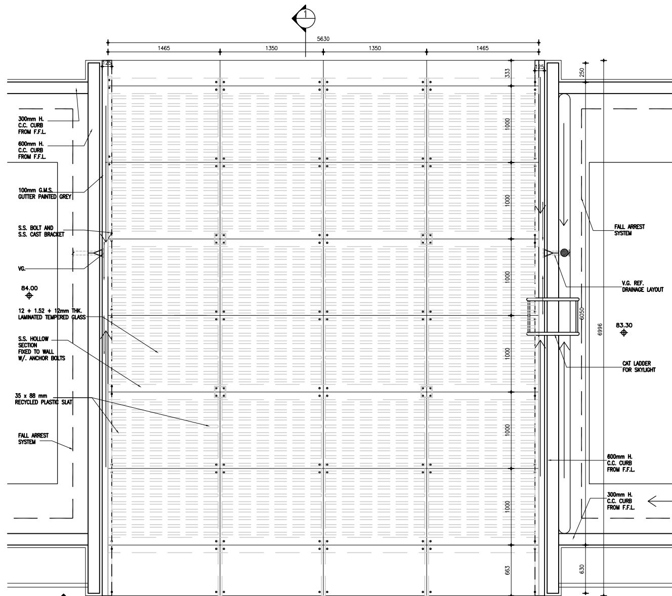
PART PLAN OF SKYLIGHT SCALE A1=1:25, A3=1:50
